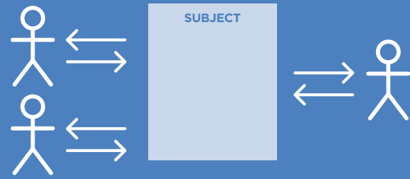
CONTEXT DIAGRAM
