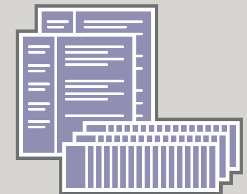
BUSINESS RULES
