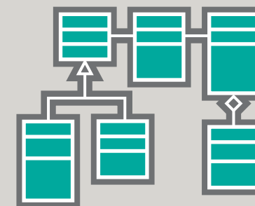
CLASS MODEL
