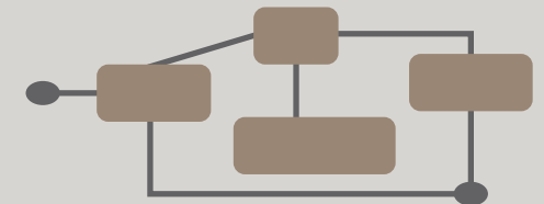
STATE DIAGRAM
