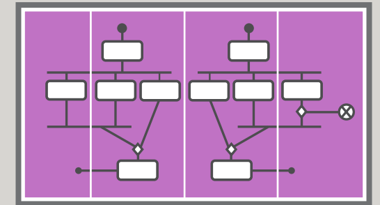
WORKFLOW MODEL
